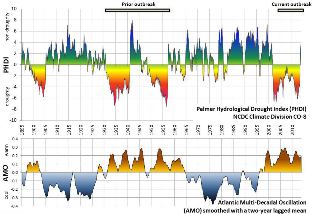
Figure 9.4—Variation in regional Palmer Hydrological Drought Index (PHDI) for northwestern Colorado and its relationship to outbreaks of the spruce beetle ( Dendroctonus rufipennis ). Regional drought is strongly influenced by hemispheric-scale variation in sea surface temperatures, particularly the Atlantic Multi-decadal Oscillation (AMO).
