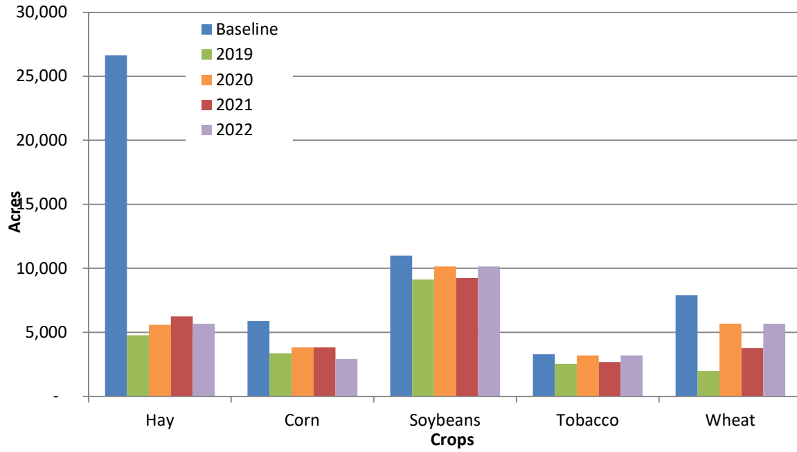
Figure 4. Reported Acreage of Major Crops from CY2019 through CY2022, compared to Baseline (CY2006), Falls Lake Watershed
